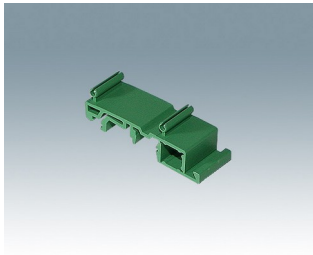
CIME/M/FE0000E RAILTEC SUP. EXT 72, DIN rail foot PA66 (UL 94 V-0) green 20.5x12.5x60mm
