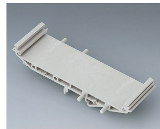
B6724443 RAILTEC SUP. 107, intermediate p. + foot PA 6 (30) (UL 94 V-0) light grey 118x35x27.5mm
