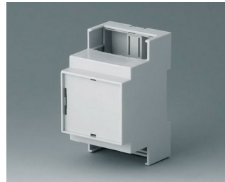
B6702106 RAILTEC C, 3 modules, Vers. IV PC (UL 94 V-0) light grey 53x90x58mm
